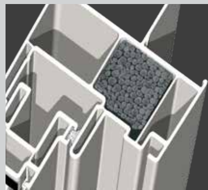
ClimaTech iE option features insulating foam liners in select mainframe channels.
